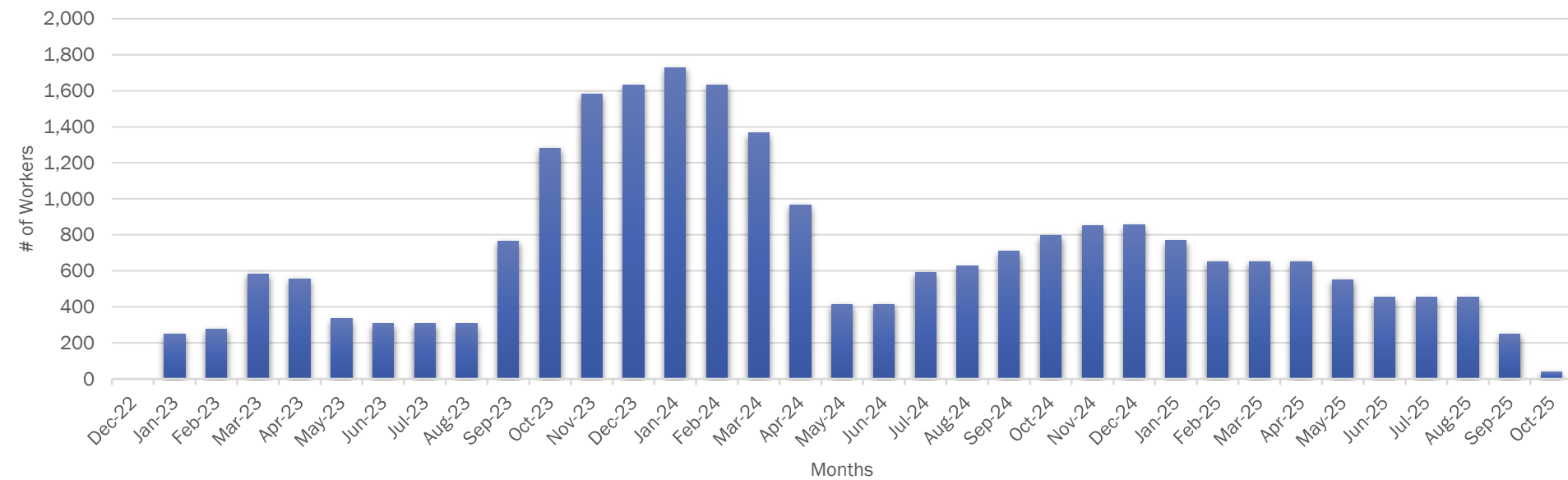
Labor Histogram: Construction & Commissioning
